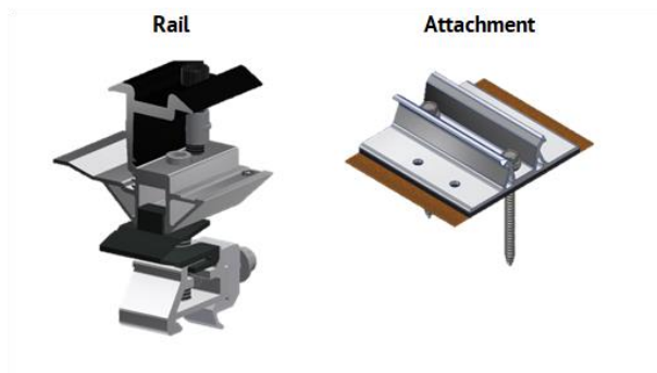
Micro Rail - DtD Rafter
