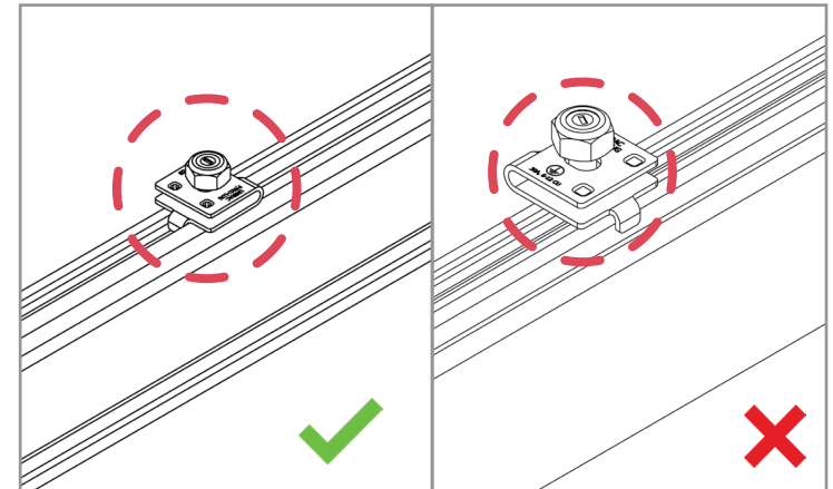
GROUNDING LUG CLIP TABS INSIDE THE RAIL
