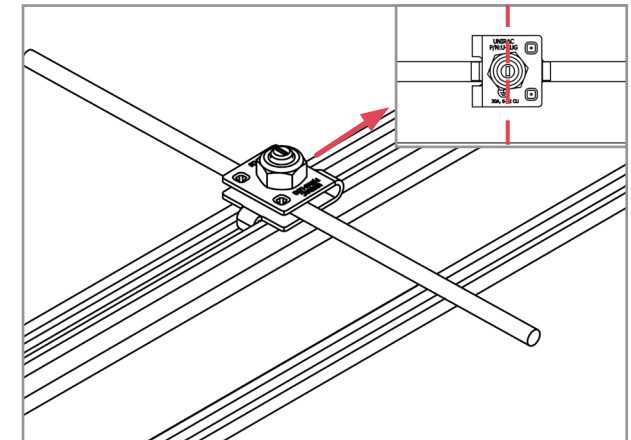
GROUNDING LUG CLIP TABS INSIDE THE RAIL
