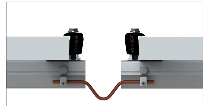
Bonding connection is used at a thermal break. Option shown uses two Ilco lugs (Model No. GBL-4DB P/N GBL-4DBT - see product data sheet for more details) and solid copper wire.
