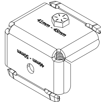
310821 - ENDCLAMP
