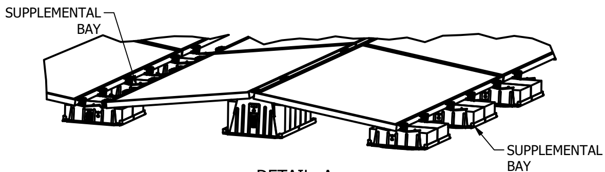
DETAIL A
