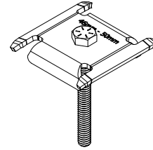
310823 - MID CLAMP
