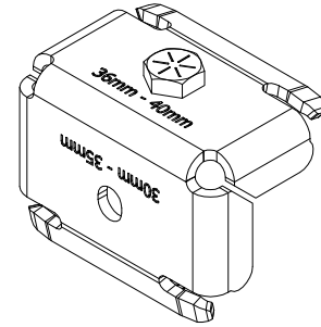
310820 - ENDCLAMP
