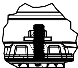
DETAIL D
