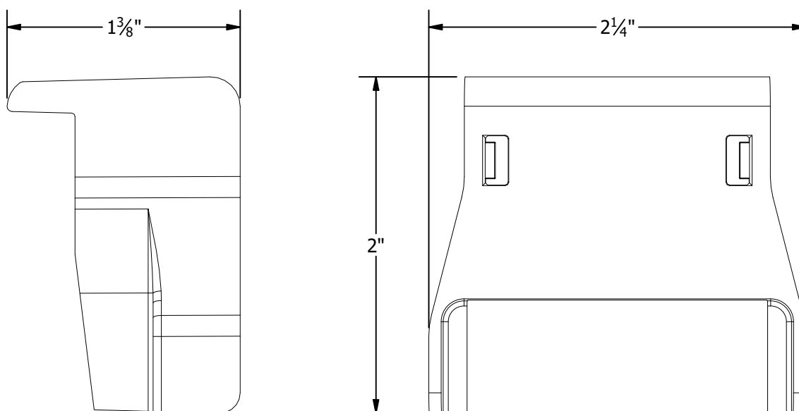
COMBO CLAMP CAP
