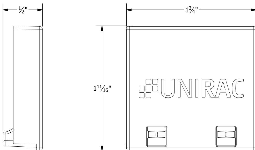
RAIL END CAP
