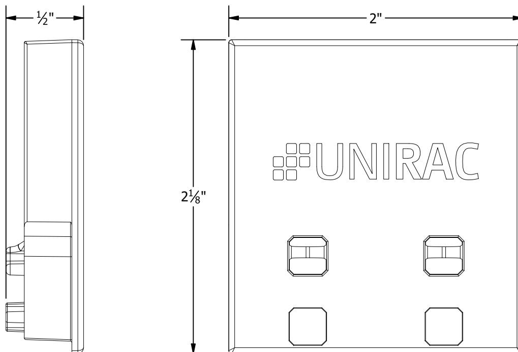
HD RAIL END CAP
