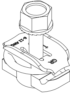
MLPE & GROUNDING ASSEMBLY SEE PAGE NU-08
