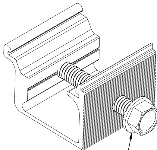
5/16"-18 x 2" SERRATED FLANGE HEX SCREW
