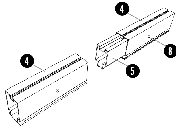
East-West Beam Splice
