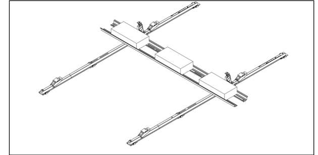
3-Block Configuration
