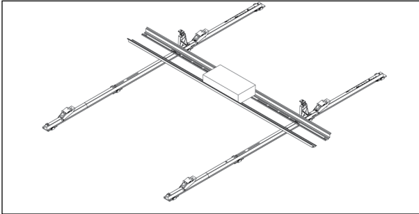
1-Block Configuration
