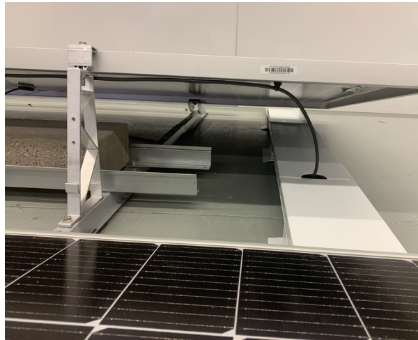
OPTION 1: USING RAYTRAY
