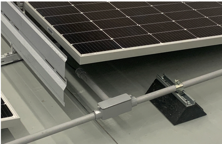
OPTION 2: USING RIGID NONMETALLIC CONDUITS
