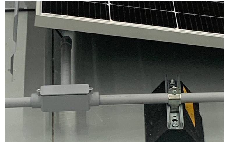
OPTION 2: USING RIGID NONMETALLIC CONDUITS
