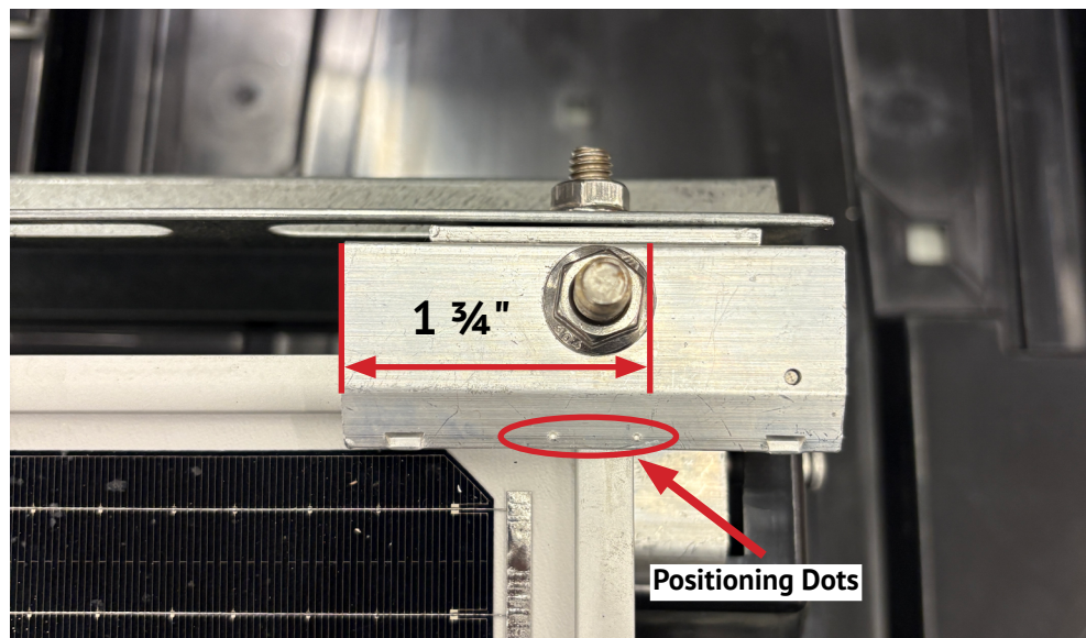
Clamp Securing Single PV Module
